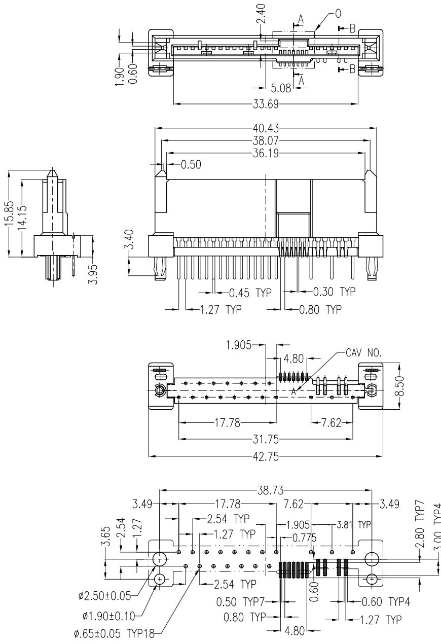
PCB LAYOUT TOP VIEW (PCB THICKNESS= Dim "B")
