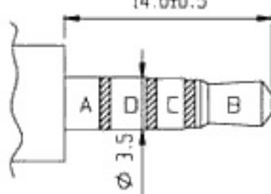
MATING PLUG
