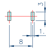
PCB Layout
